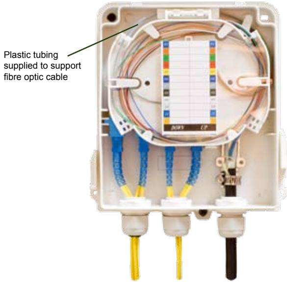
Open view
